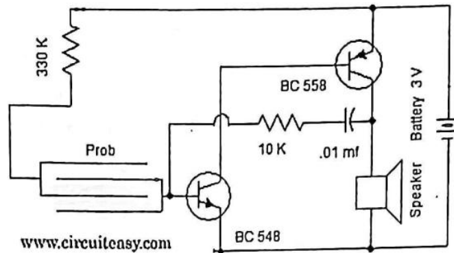
Circuit Diagram of Rain Alarm
