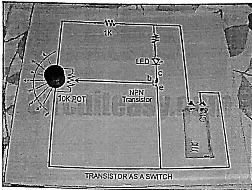
Transistor as a switch
