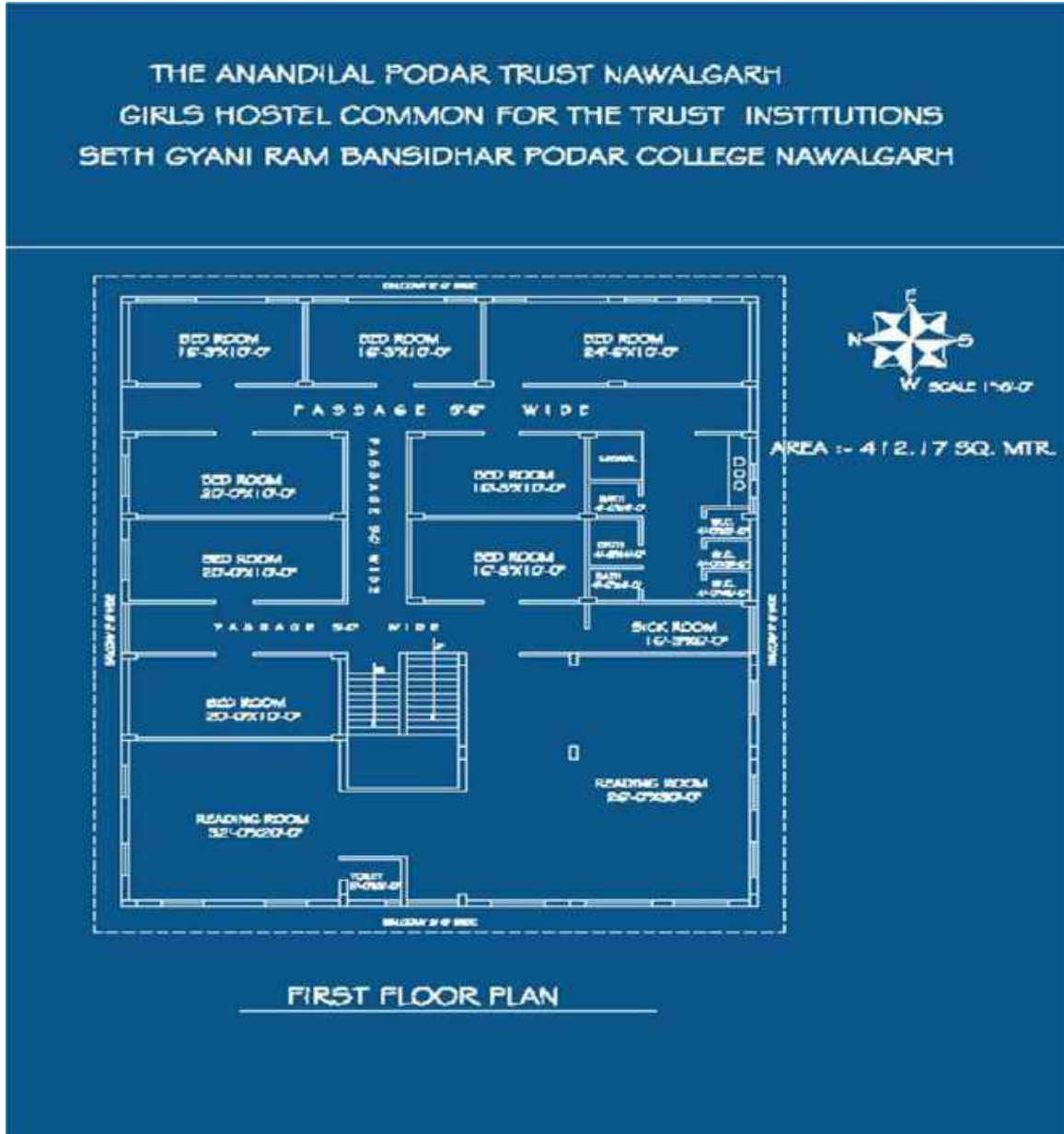
Girls Hostel First Floor
